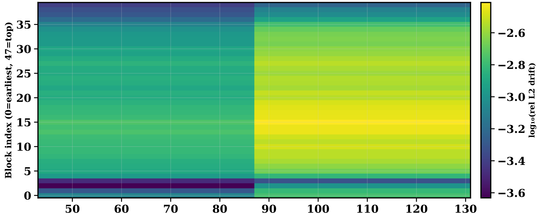
m09c stage1_layout step=131 · Per-block weight drift vs Meta init (rows=blocks, cols=val checkpoints)
